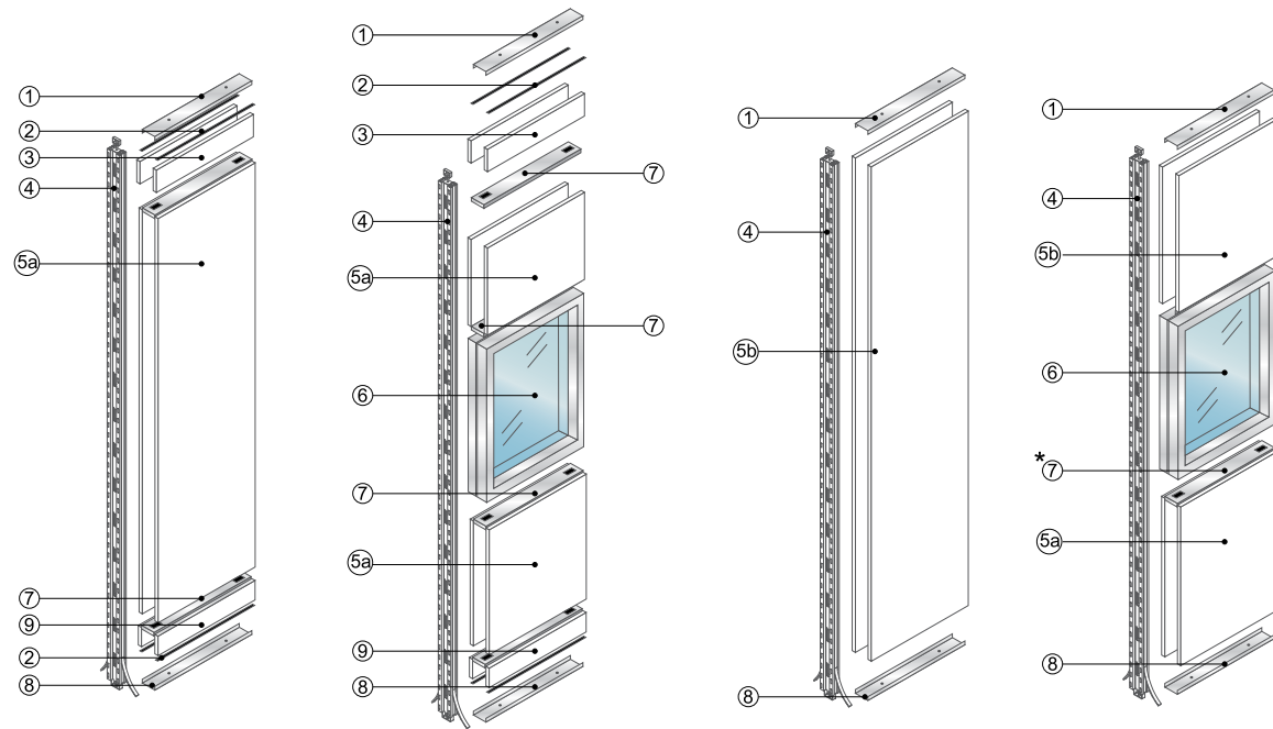
WALL SYSTEM 1
